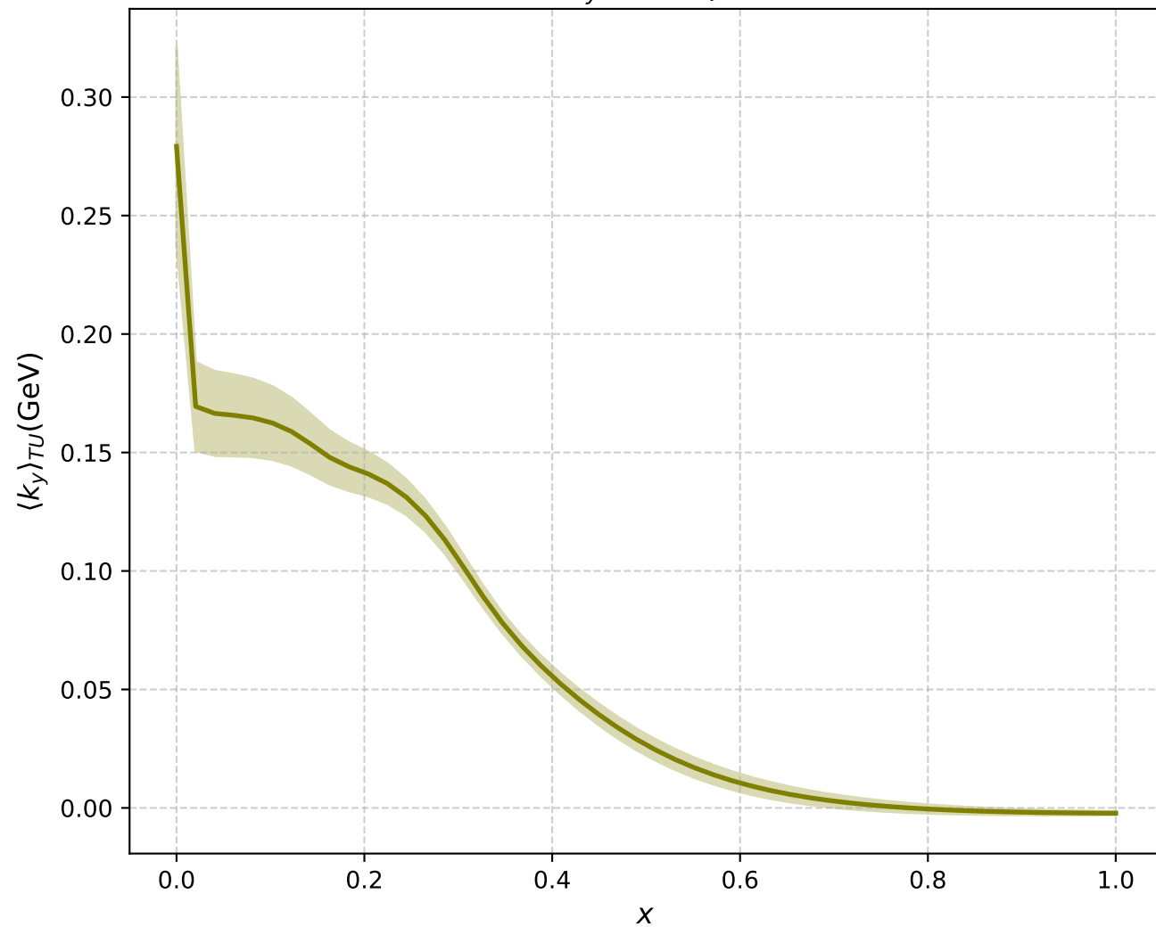
Sivers Shift \langle k_y \rangle_{TU} ( 1/\hat{\zeta} \rightarrow 0 , b^2=9.0 )
