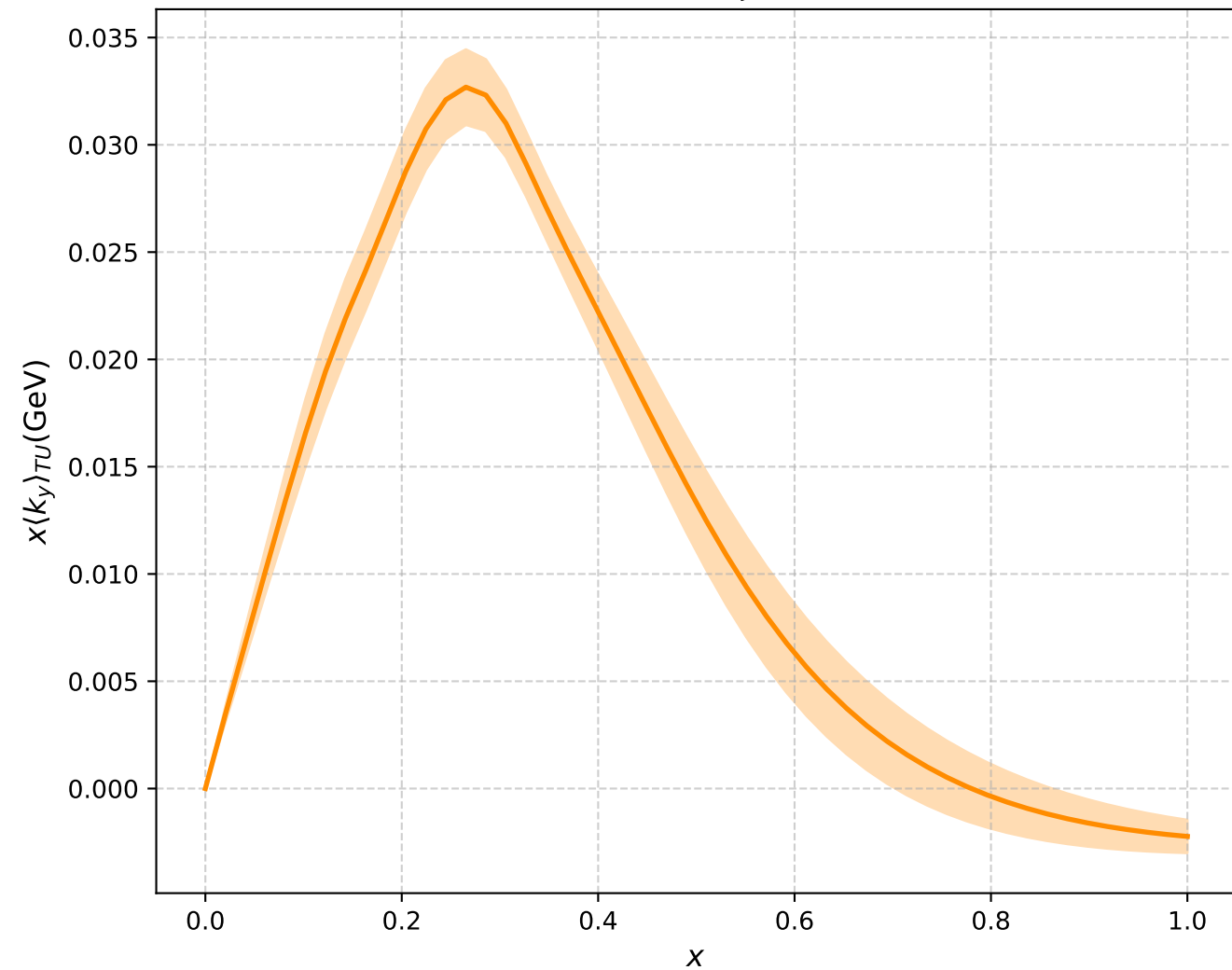
x^* Sivers Shift ( 1/\hat{\zeta} \rightarrow 0 , b^2=9.0 )
